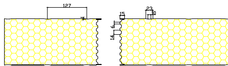
Panel Connection Detail
