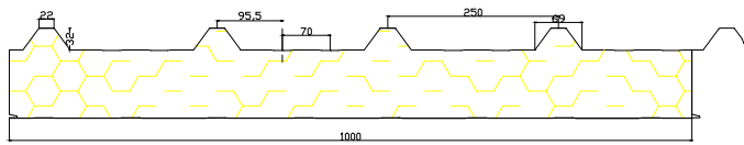
Panel Detail
