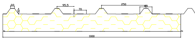
Panel Detail
