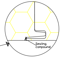
Sealing Compound Flush With Panel
