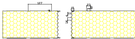
Panel Connection Detail
