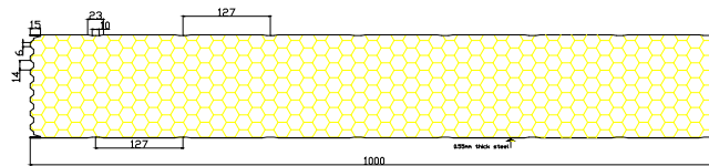
Panel Profile
